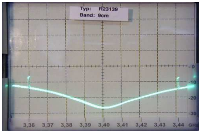
SWR 9cm
